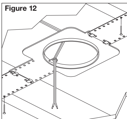
Figure 12 The optional hole saving brackets are installed and the loudspeaker wire is attached to the bracket.
